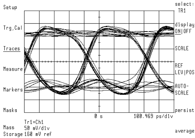
Example Filtered Laser Overshoot
