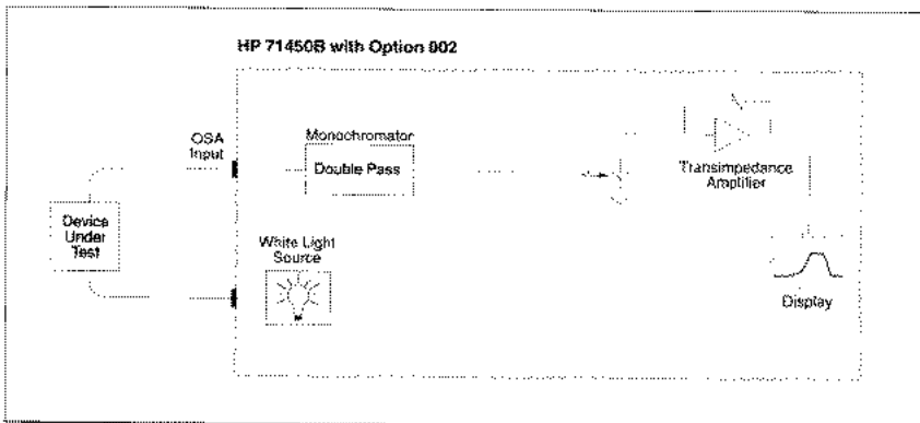
Figure 6. Stimulus response measurement setup
