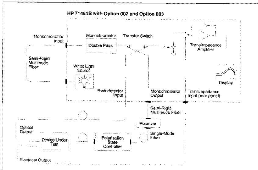
Figure 7. Swept PDL measurement setup
