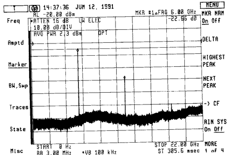
Figure 2. Harmonic distortion on an analog modulated laser
