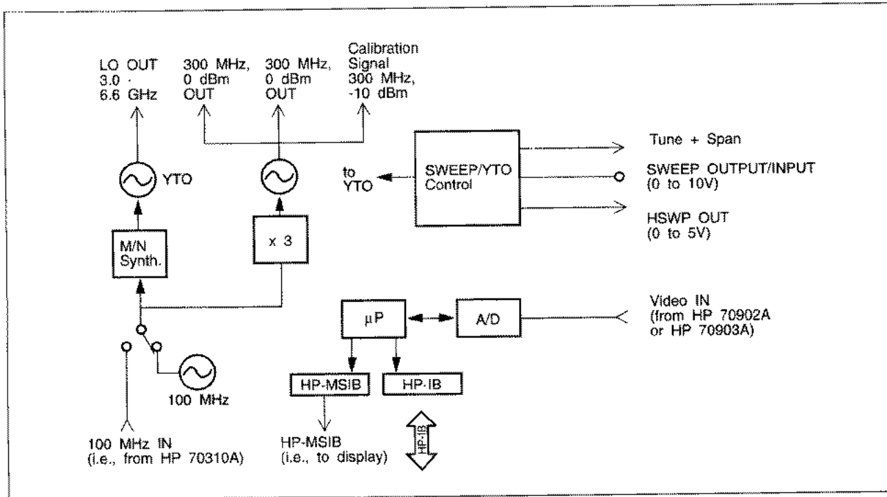
HP 70900B local oscillator/control module block diagram
