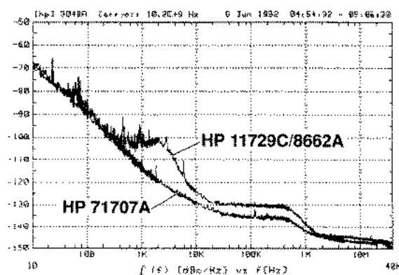
Typical phase noise of HP 71707A and HP 11729C carrier noise test set, using the HP 8662A as a reference
